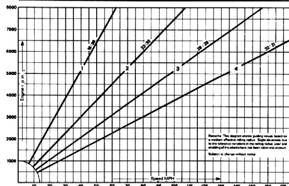
Transmission Diagram Turbo 4-speed-transmission
