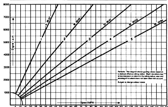
Transmission Diagram 911 SC 5-speed-transmission
