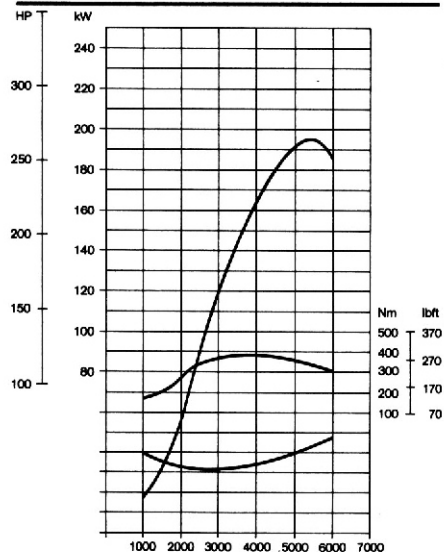
Full-Power Performance Turbo
