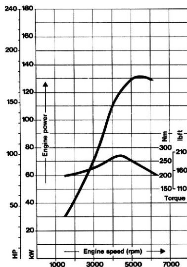
Full-power Curve SAE
